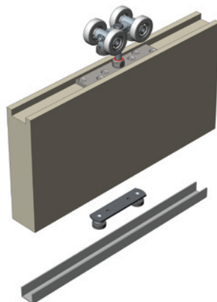
GUIDE CHANNEL IN FLOOR
